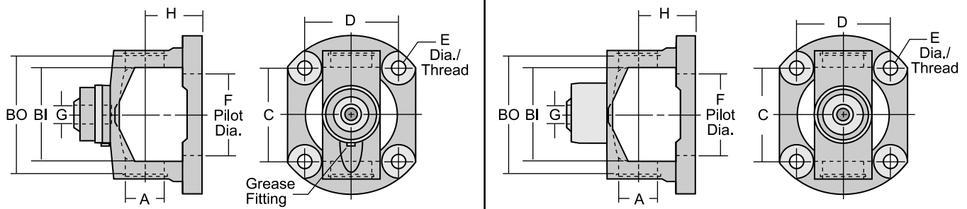
Type 1 (External Seal)
