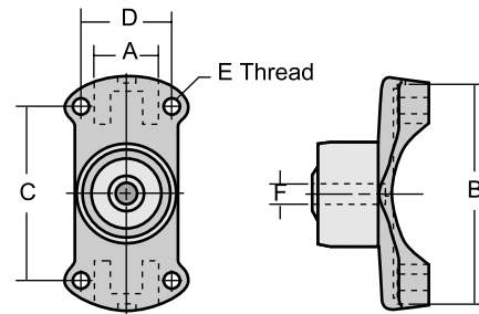
Type 2 (Internal Seal)
