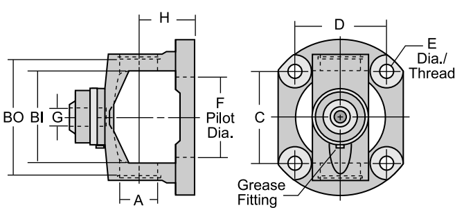
Type 1 (External Seal)
